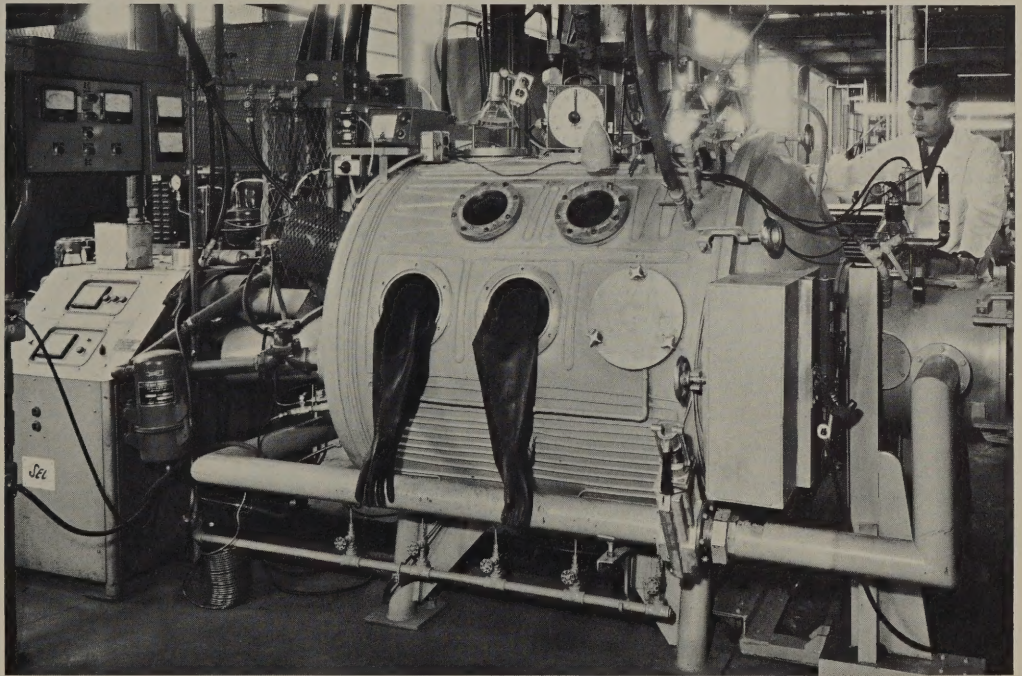
Gypsum plants like this one at left contribute to Nevada's sizable mineral output. Scientists use this machine (below) at the Reno Metallurgy Research Center to develop new processing and mining techniques that will sustain the State's ever-increasing mineral yields in the years to come.
